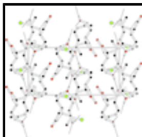
Fig. 2. : Packing view showing the C–H···O hydrogen bonds as dashed lines. H atoms not involved in hydrogen bonding have been omitted for clarity.
